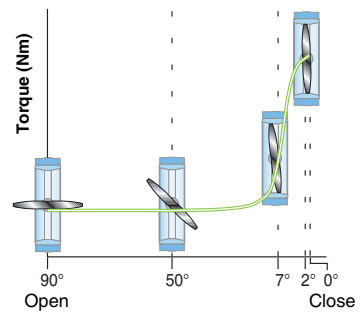
Butterfly valve
