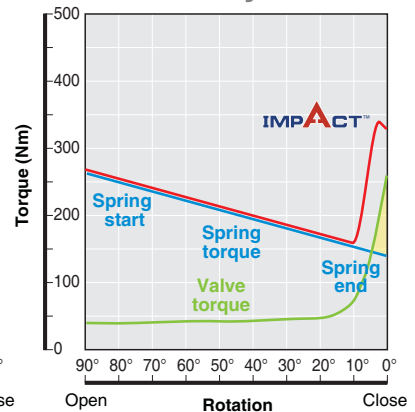
Butterfly valve
