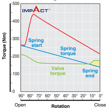
Plug valve
